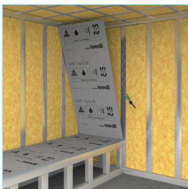
wedi Vapor 85 is direct bonded onto metal stud frames with the use of wedi 610 adhesive sealant...
